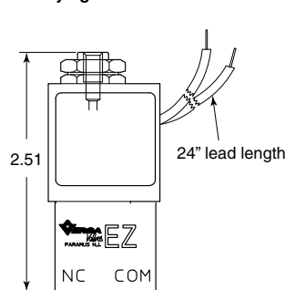
Flying Leads
